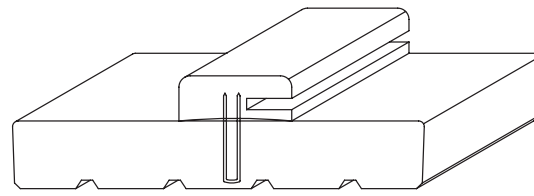
Applied Stop Jamb Kerfed for weatherstrip
