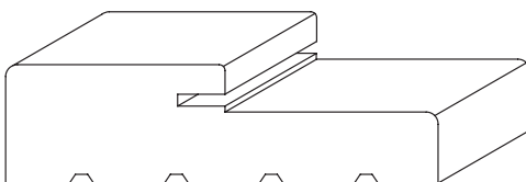
Exterior Jamb, kerfed with weatherstrip
